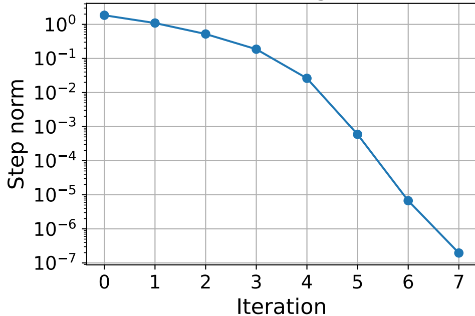
SQP convergence
